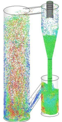
Combustion simulation of municipal solid wastes using the representative particle model. During the combustion process, the solid waste particles reduce to micron-order ash and various gases are generated and extinguished
