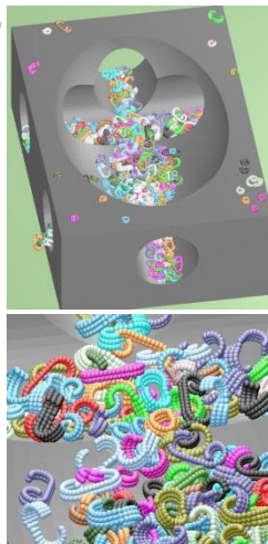
Combustion simulation of municipal solid wastes using the representative particle model. During the combustion process, the solid waste particles reduce to micron-order ash and various gases are generated and extinguished
